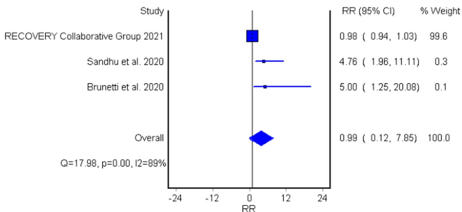
Fig. 5 Forest plot for the efficacy of colchicine on hospital discharge rate in patients with COVID-19
